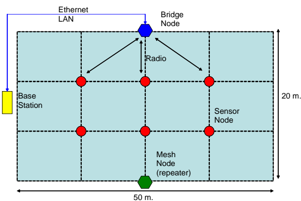
Figure 2. Sensors field structure for the experiment
